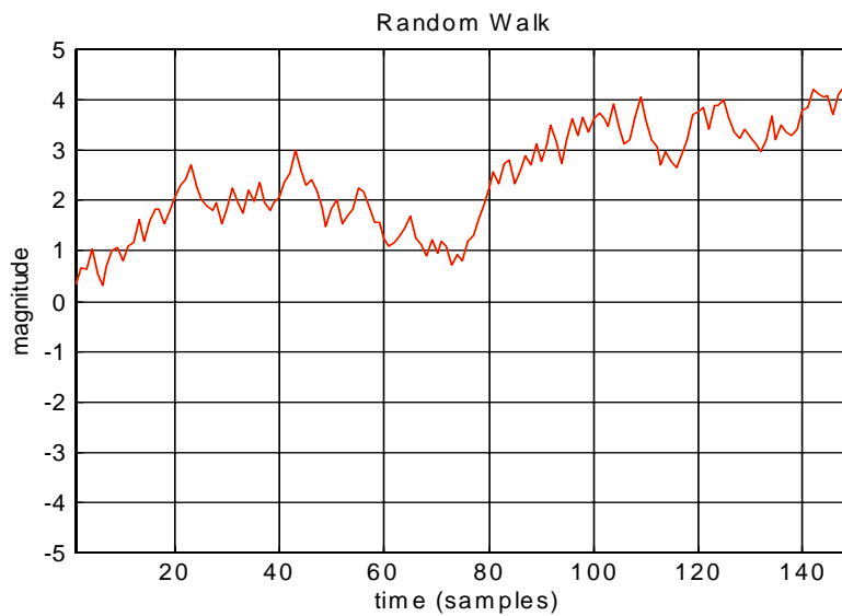
Figure 5-3 Random Walk
